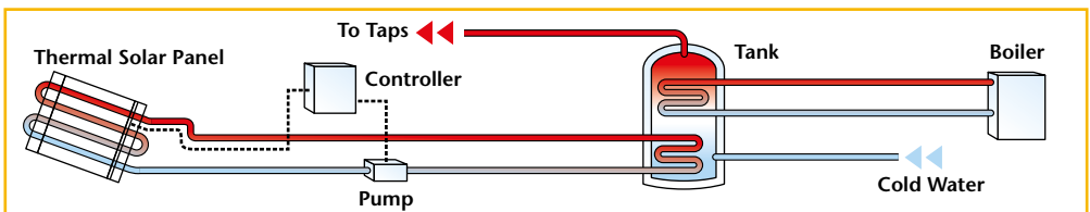
Typical Evacuated Tube/ Flat Plate Solar Collector system
